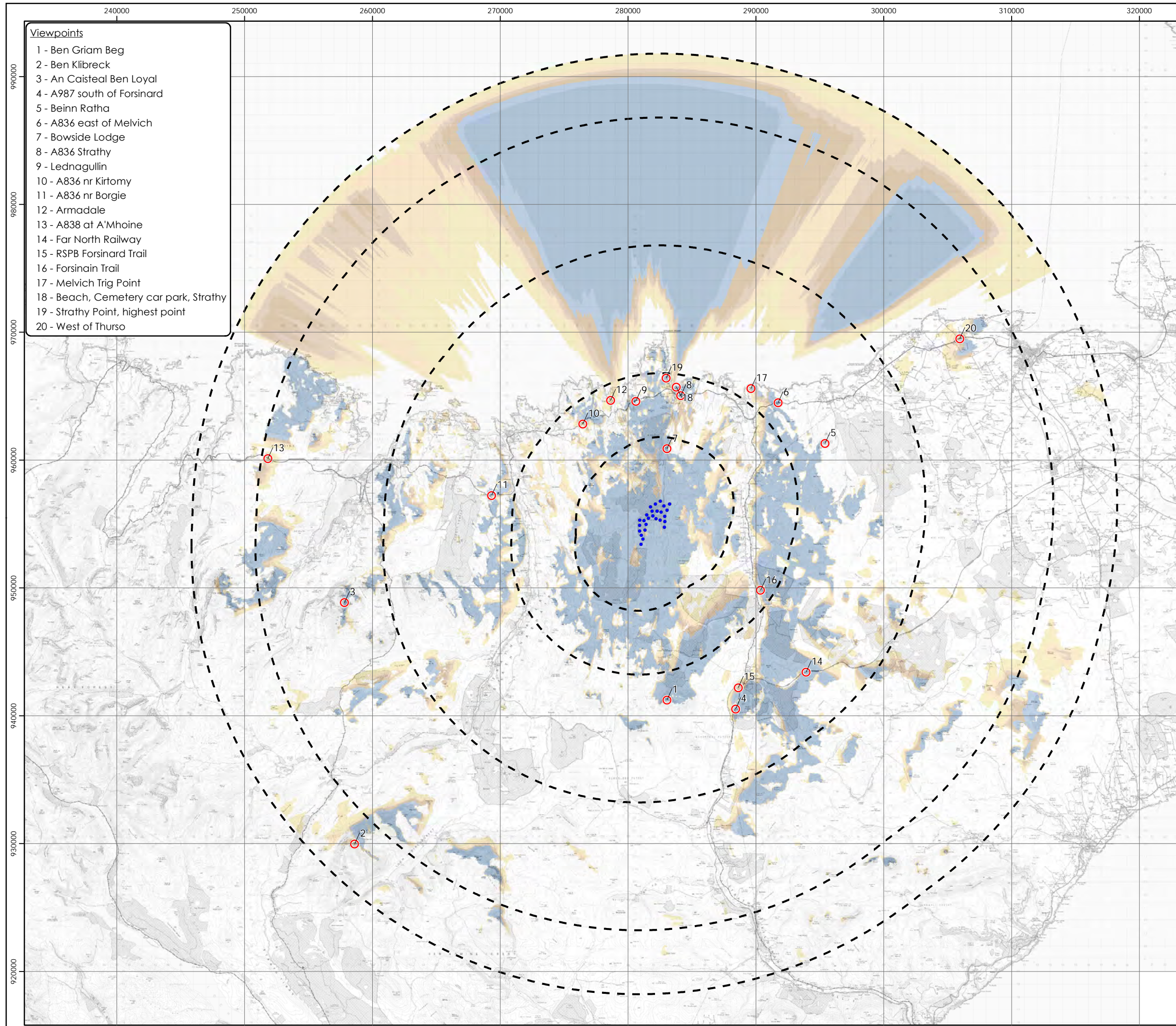
Figure 7-4 Blade Tip Unscreened ZTV at 35km radius with Viewpoints
