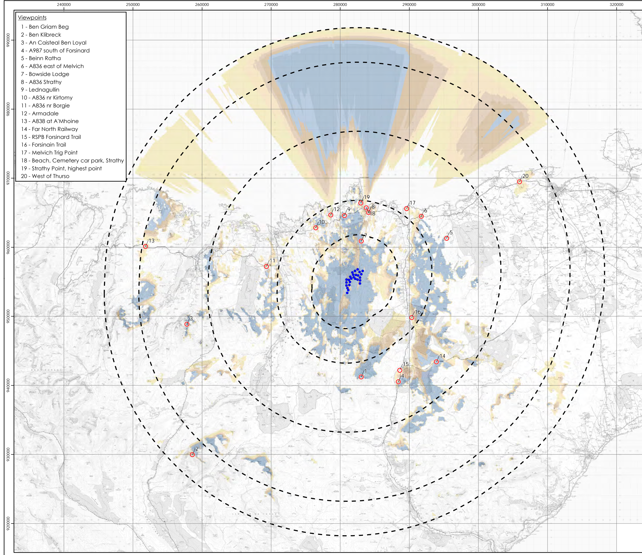
Figure 7-5 Hub Height Unscreened ZTV at 35km radius with Viewpoints
